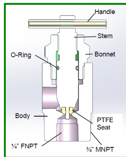
Model 331 Drawing
